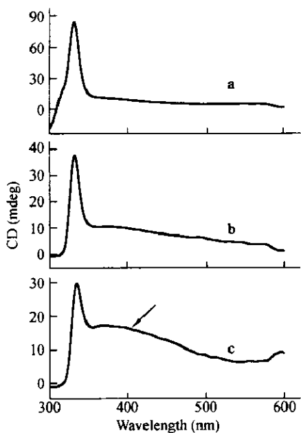
Fig. 7 CD spectra of PhthCS/DMAc solutions with varying concentration a) 41 %; b) 42 %; c) 43 %
