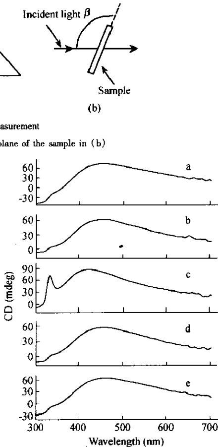
Fig. 10 CD spectra of 45% PhthCS/DMAc solution with different \beta a) \beta = 60^\circ ; b) \beta = 75^\circ ; c) \beta = 90^\circ ; d) \beta = 105^\circ ; e) \beta = 120^\circ
