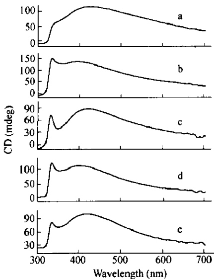
Fig. 9 CD spectra of 45% PhthCS/DMAc solution with different \alpha a) \alpha = -30^\circ ; b) \alpha = -15^\circ ; c) \alpha = 0^\circ ; d) \alpha = +15^\circ ; e) \alpha = +30^\circ
