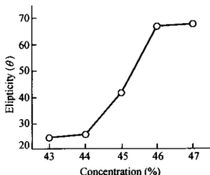
Fig. 3 The relationship between concentration and ellipticity of PhthCS/DMF solution ( \lambda = 410 \text{ nm} )
